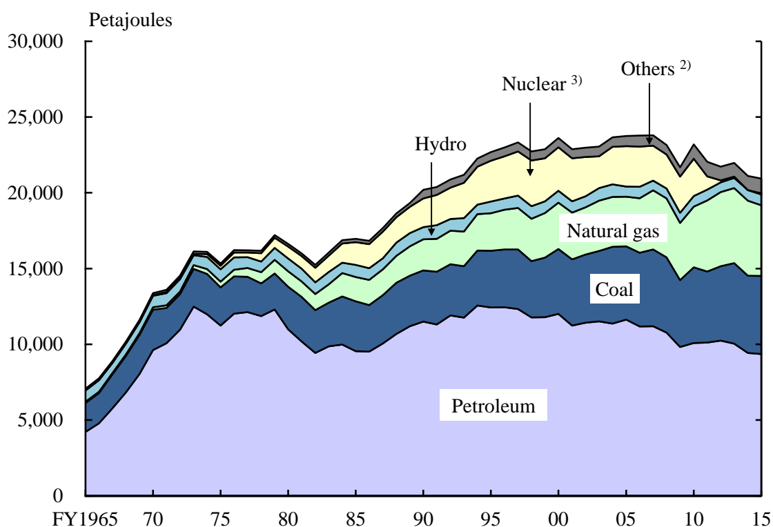
Figure 7.1 Total Primary Energy Supply 1)
